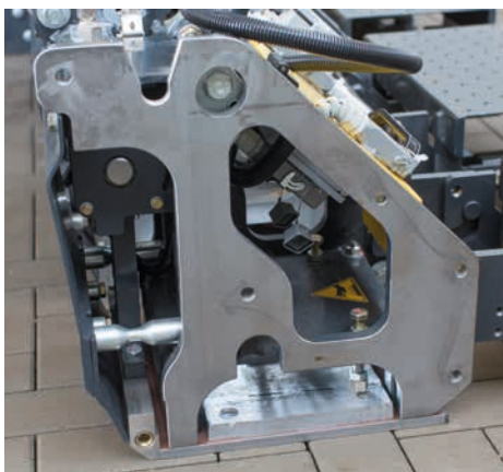
Surprisingly simple: Heating system with monitored heating circuits.
