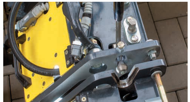
Brilliantly simple: The receptacle of the QUICK COUPLING system.
